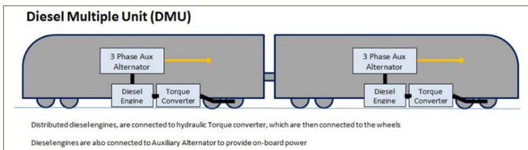
Figure 5-1: Characteristics of a DMU with diesel-hydraulic transmission
