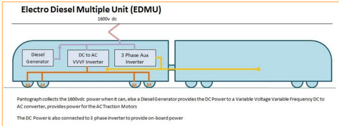
Figure 5-2: Characteristics of an EDMU
